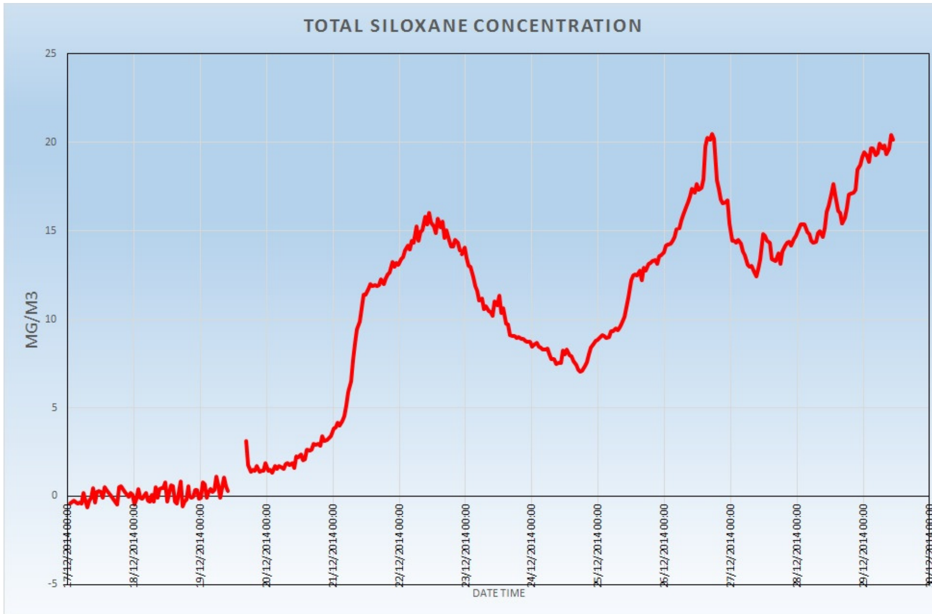
Siloxane breakthrough in a Carbon Filter removal system
